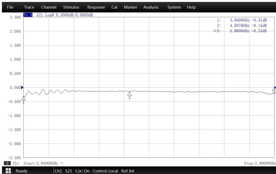
Insertion Loss*
